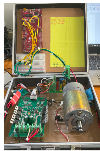
c) TMS320F28379
